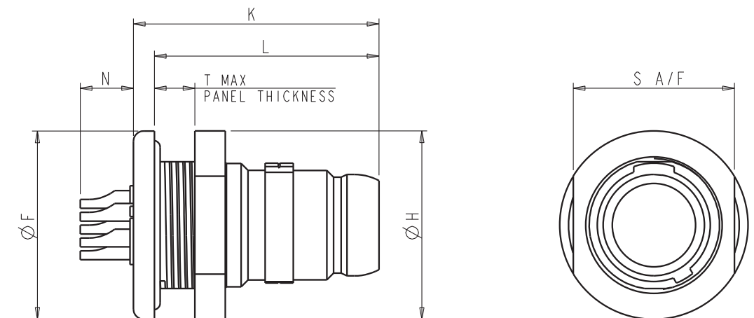
SOLDER BUCKET TYPE (-002)
